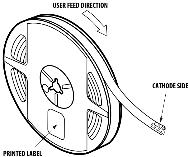
Figure 26. Reeling Orientation.
