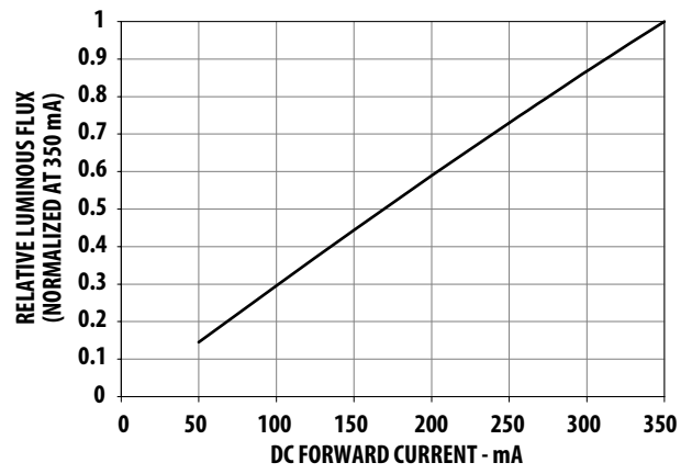
Figure 2. Relative Luminous Flux vs. Mono Pulse Current.
