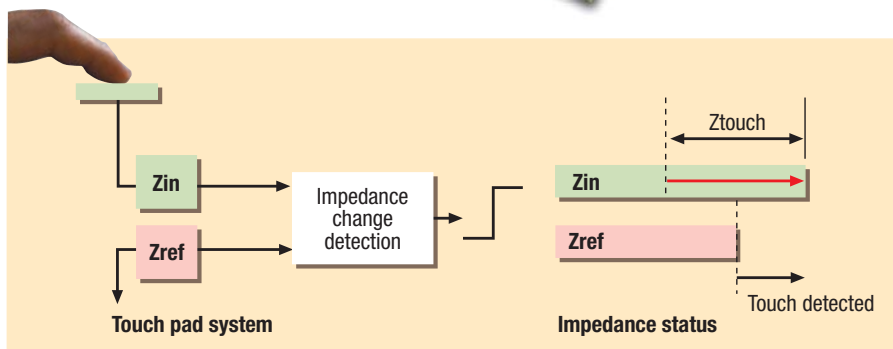
Principle of touch detection
