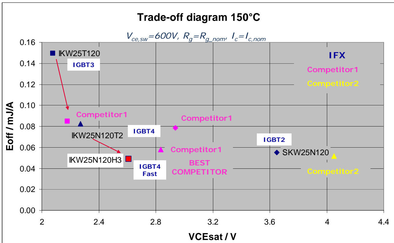
Fig 5: trade-off V_{cesat} - E_{off}
