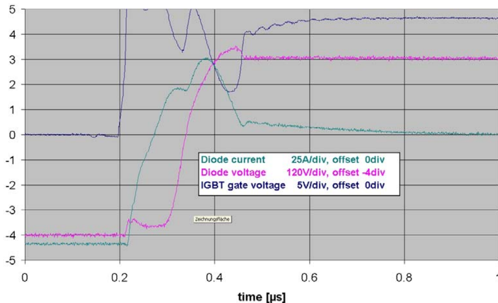
Fig 6: Diode commutation at extreme switching conditions.
