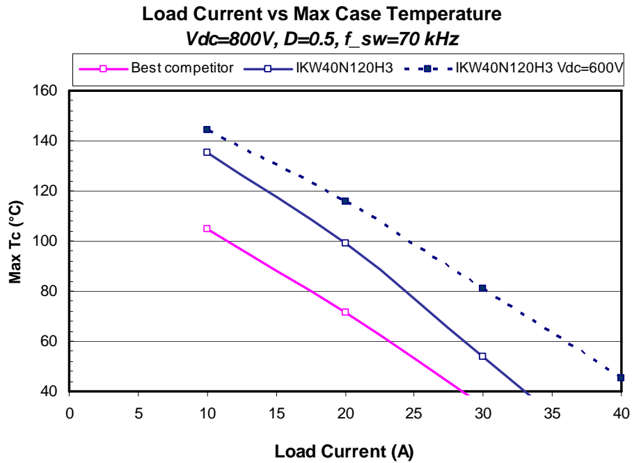
Figure 12: max load current at f_{sw}=70 kHz and dependence on bus Voltage V_{dc} .
