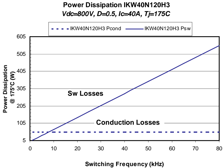
Fig.10: breakdown of switching vs conduction losses.
