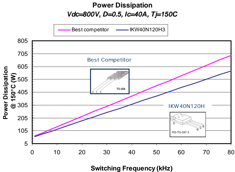
Fig 9: Total losses of IKW40N120H3 (TO247) and Best Competitor (TO264)
