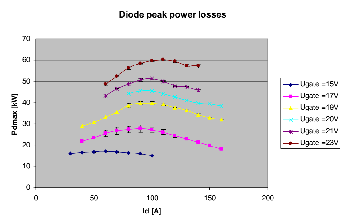
Fig.7: Diode power dissipation at IGBT Turn-on (IKW40N120H3): V_{ce}=850V , T_j (diode)=175°C,
