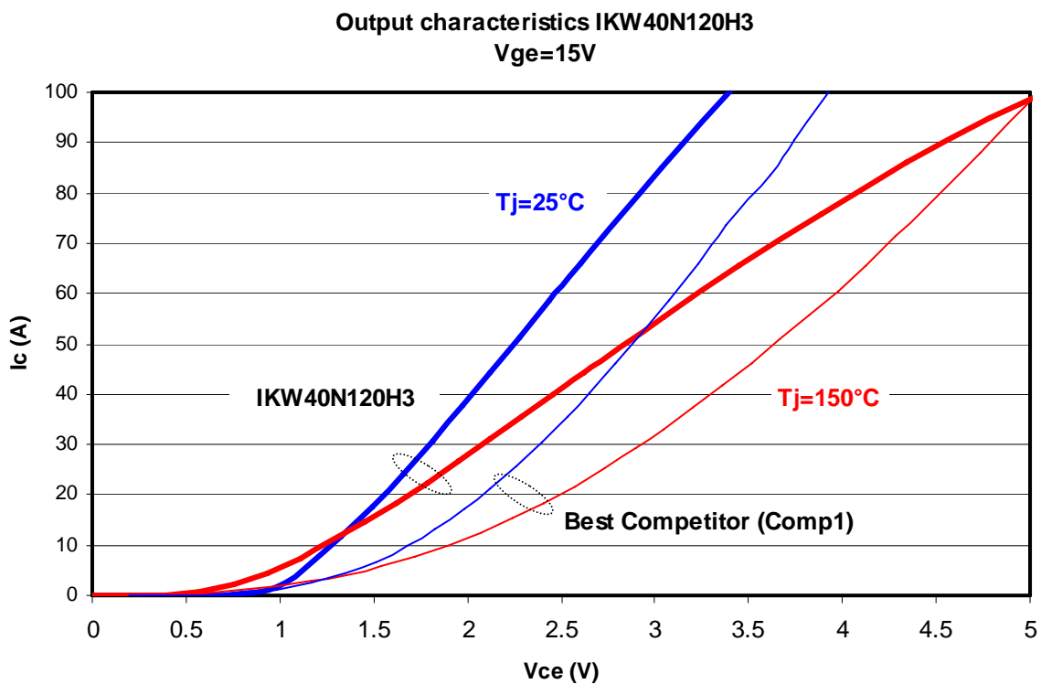
Figure 3: Output characteristics of the High Speed 3 IGBT.
