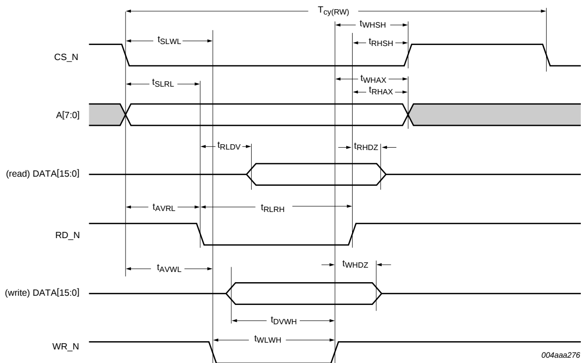
Fig 16. Register access timing: separate address and data buses
