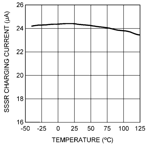
SSSR Pin Charging Current vs Temperature
