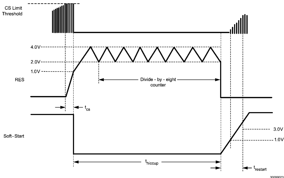
FIGURE 16. Hiccup Mode Timing
