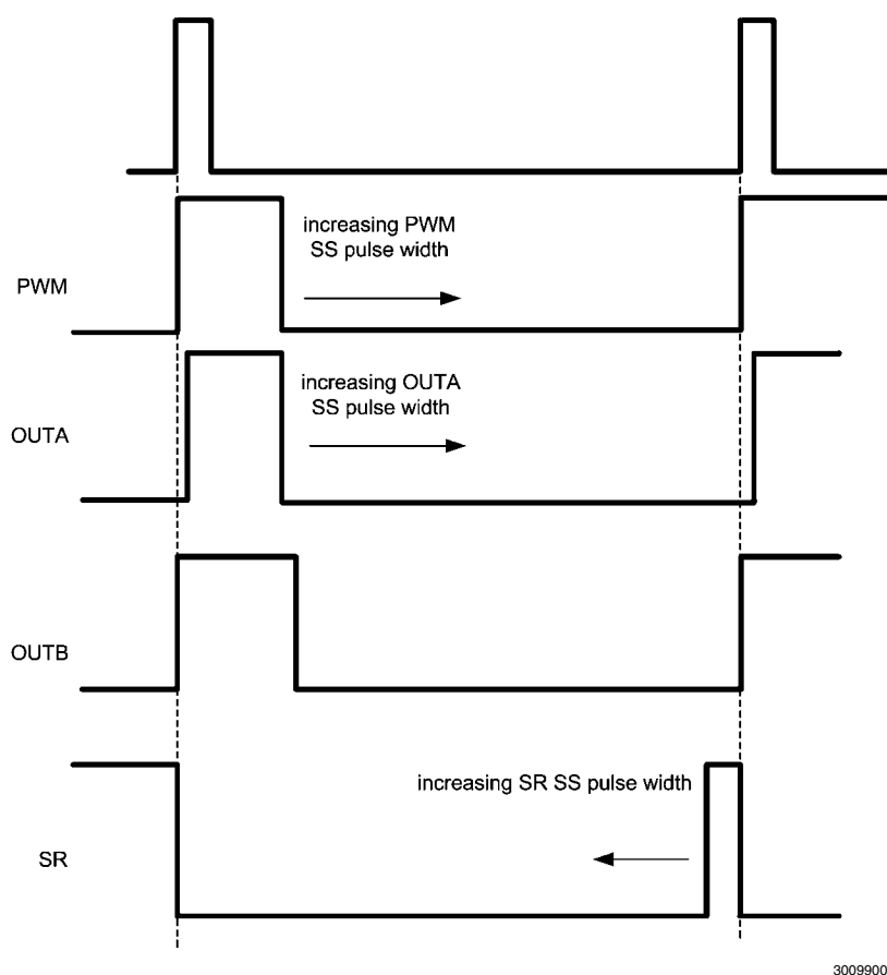
FIGURE 3. Soft-Start Timing
