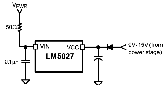
FIGURE 10. Start-up Regulator Power Reduction
