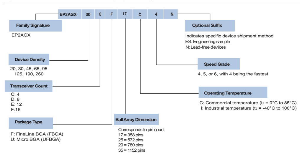
Figure 1-2. Arria II GX Device Packaging Ordering Information
