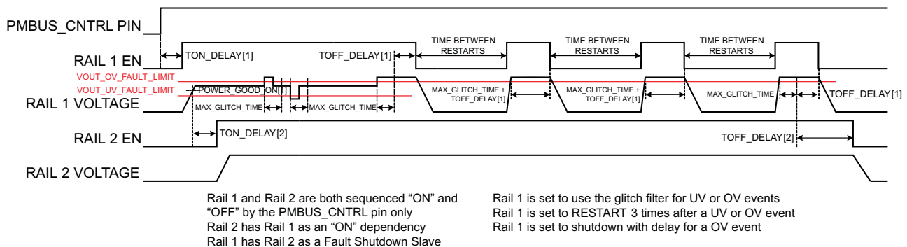
Figure 12. Sequencing and Fault-Response Timing
