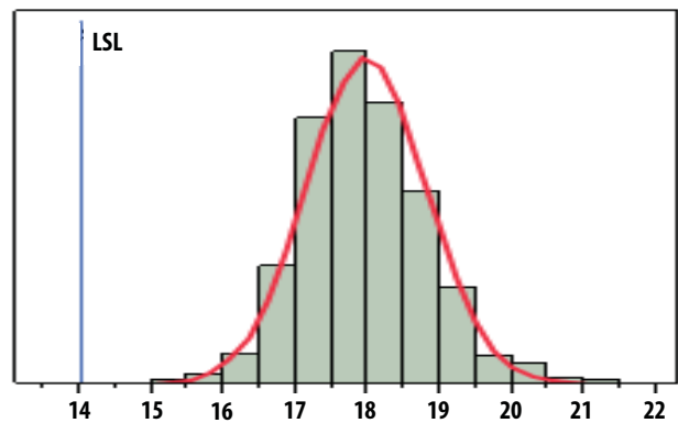
Figure 4. IIP3, LSL = 14 dB, nominal = 17.9 dB
