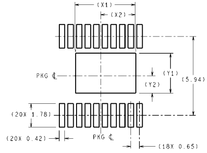
LAND PATTERN RECOMENDATION
