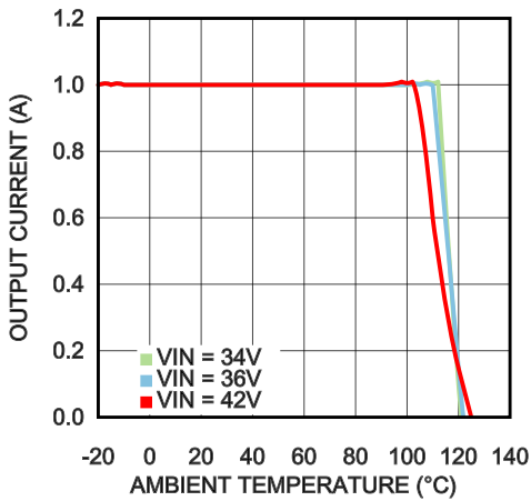
Thermal Derating V_{OUT} = 30V , \theta_{JA} = 16^{\circ}C/W
