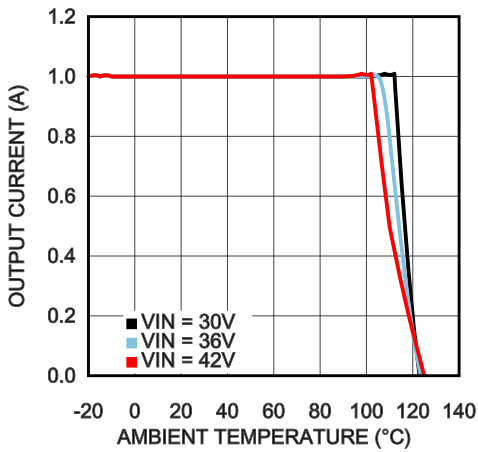
Thermal Derating V_{OUT} = 24V , \theta_{JA} = 16^{\circ}C/W
