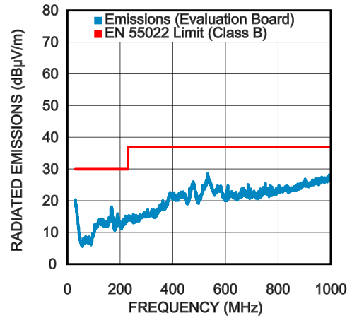
Radiated EMI of Evaluation Board, V_{OUT} = 12V
