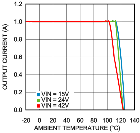
Thermal Derating V_{OUT} = 12V , \theta_{JA} = 16^{\circ}C/W
