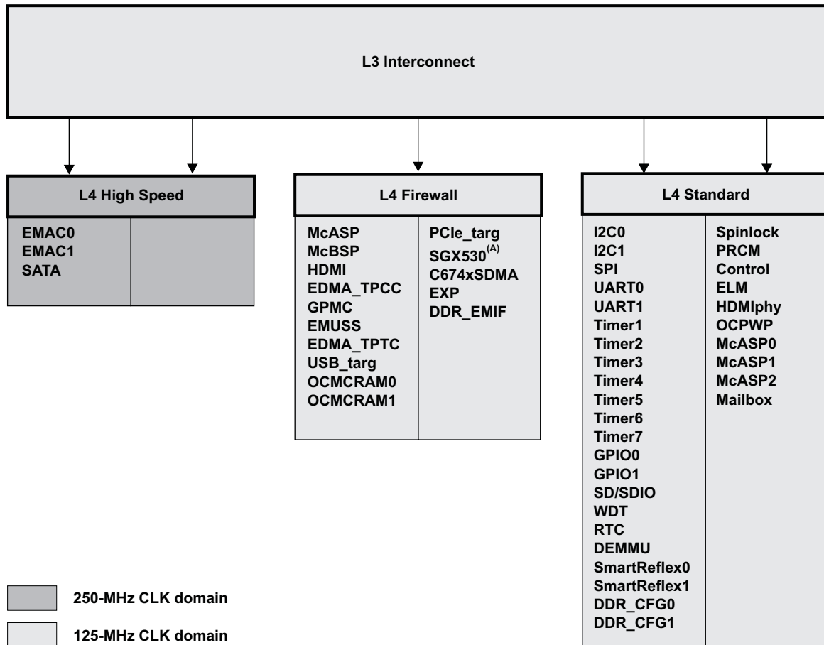
Figure 5-2. L4 Architecture
