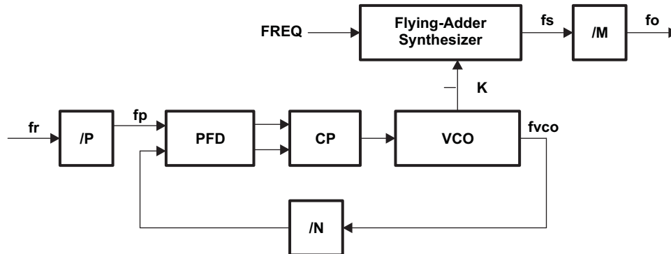
Figure 7-8. Flying-Adder PLL
