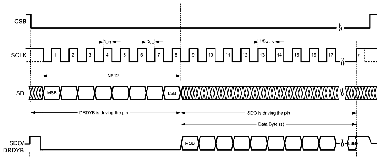
FIGURE 2. Timing Diagram
