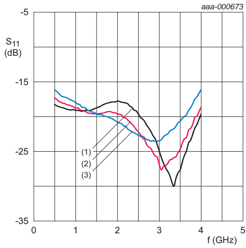
V_{SUP} = 5\text{ V} ; maximum current setting; minimum attenuation. (1) T_{amb} = -40\text{ °C} (2) T_{amb} = +25\text{ °C} (3) T_{amb} = +85\text{ °C}
