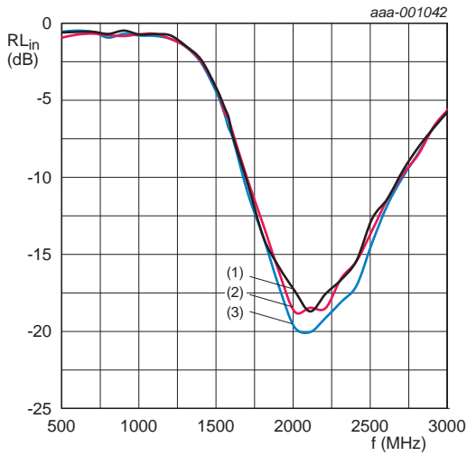
P_i = -45 dBm; T_{amb} = 25 °C. (1) V_{CC} = 1.5 V (2) V_{CC} = 1.8 V (3) V_{CC} = 2.2 V
