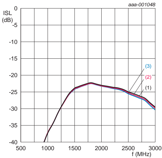
V_{CC} = 1.8 \text{ V}; P_i = -45 \text{ dBm}. (1) T_{\text{amb}} = -40 \text{ }^\circ\text{C} (2) T_{\text{amb}} = +25 \text{ }^\circ\text{C} (3) T_{\text{amb}} = +85 \text{ }^\circ\text{C}
