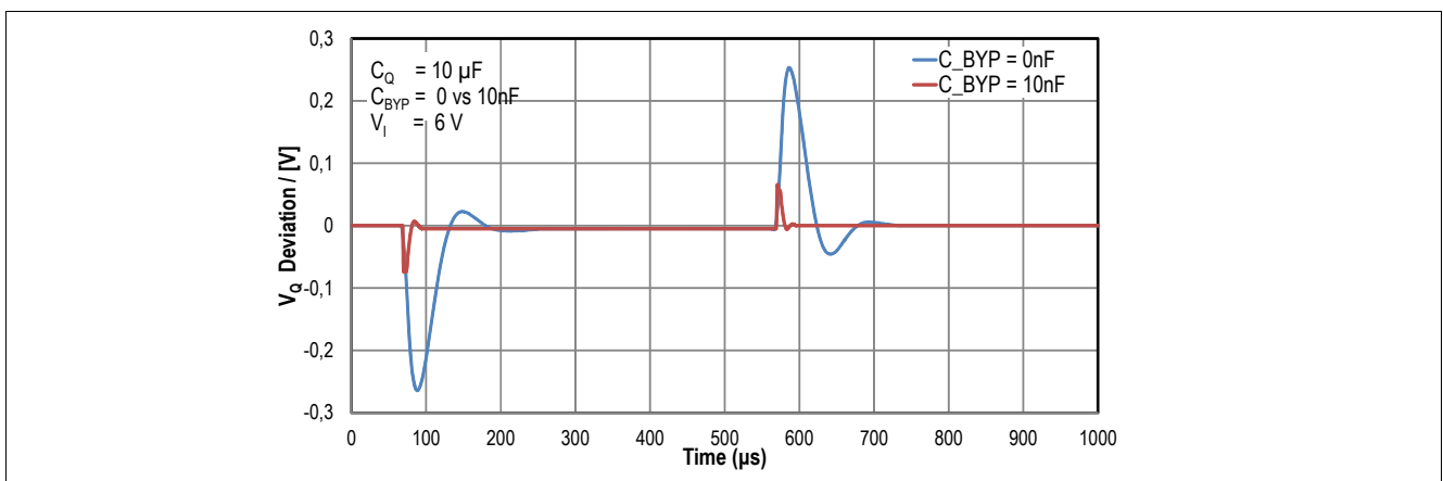
Figure 7 Influence of C_{BYP} : example of transient response to one and the same load step with and without C_{BYP} of 10 nF ( I_Q : 100 mA to 500 mA, TLS205B0EJV33)
