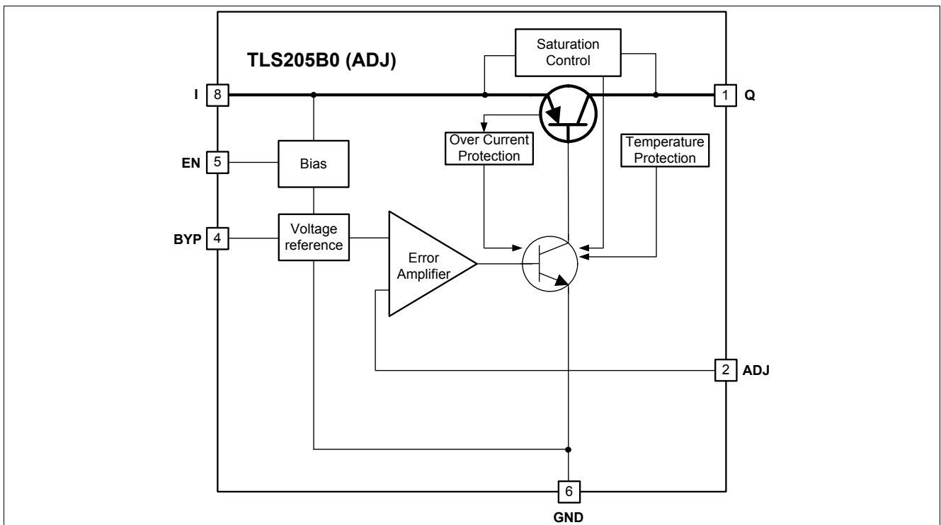
Figure 2 Block Diagram TLS205B0 adjustable version
