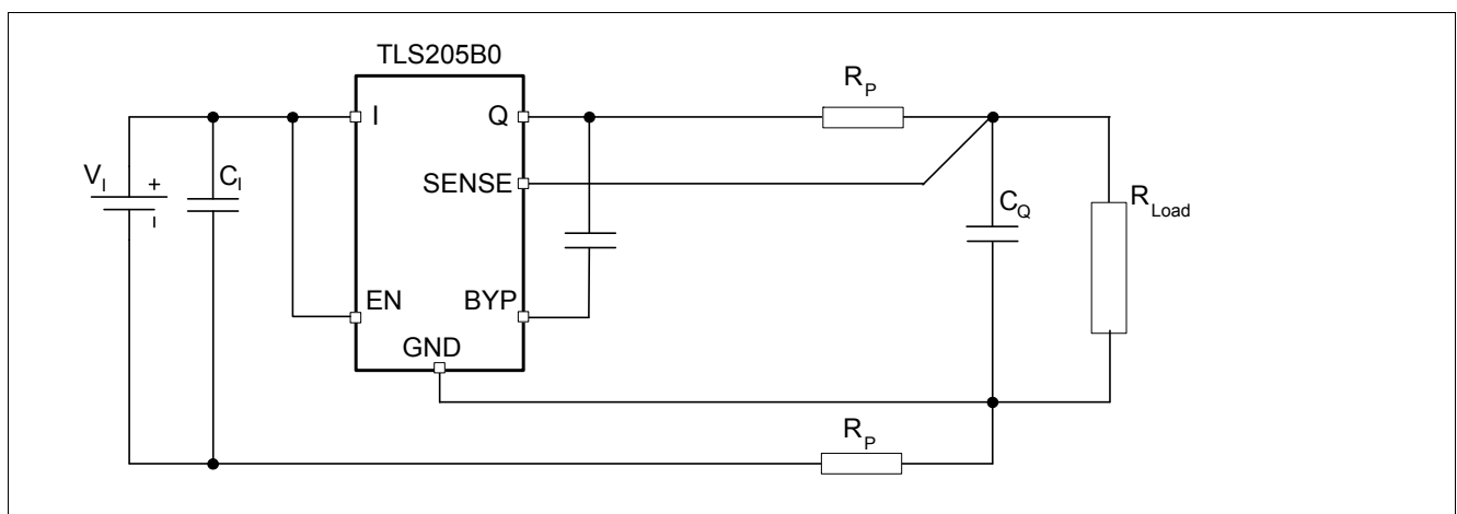
Figure 6 Kelvin Sense Connection
