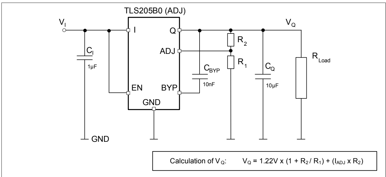
Figure 5 Typical Application Circuit TLS205B0 (adjustable version)
