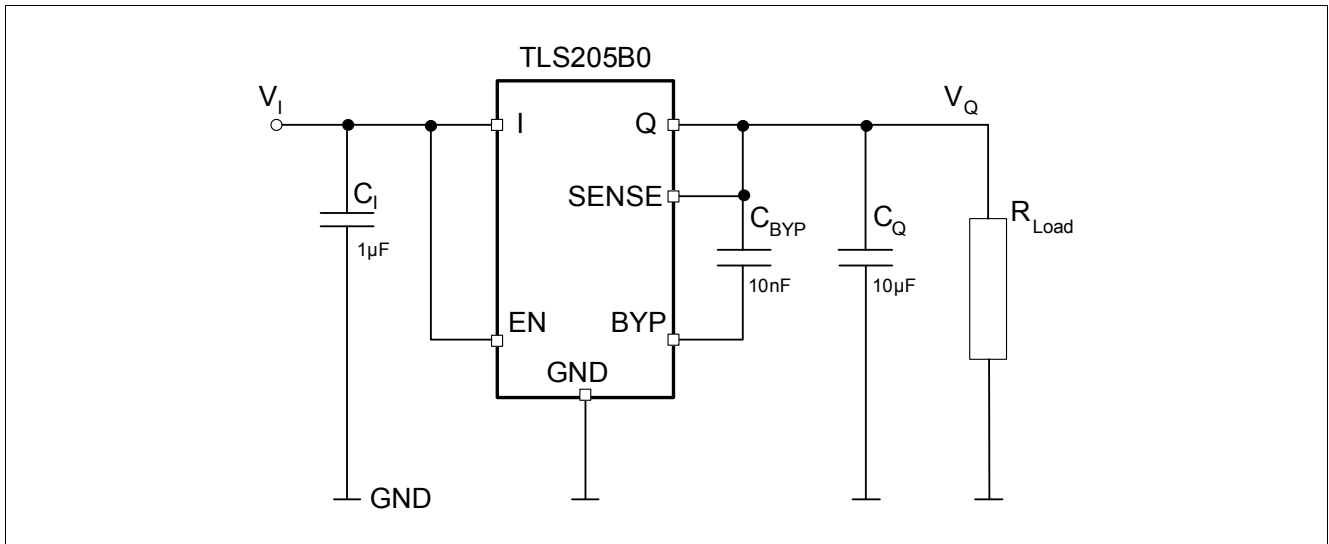
Figure 4 Typical Application Circuit TLS205B0 (fixed voltage version)
