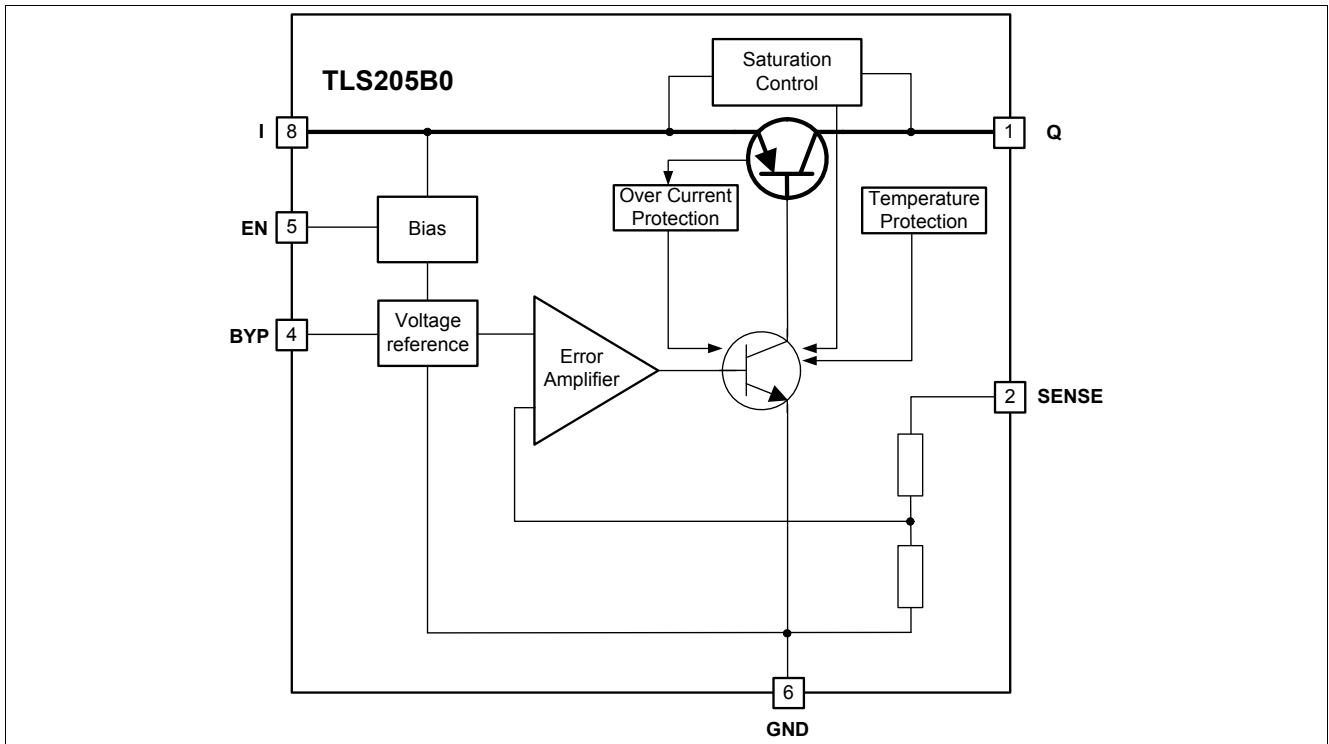
Figure 1 Block Diagram TLS205B0 fixed voltage version
