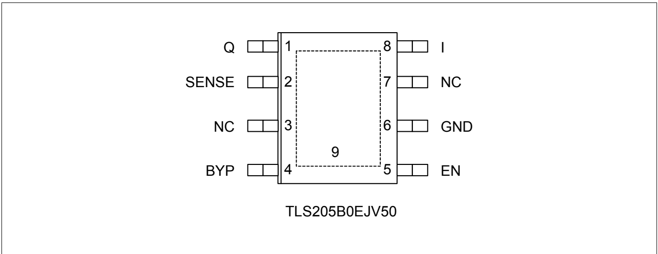
Figure 2 Pin Configuration of TLS205B0EJV50
