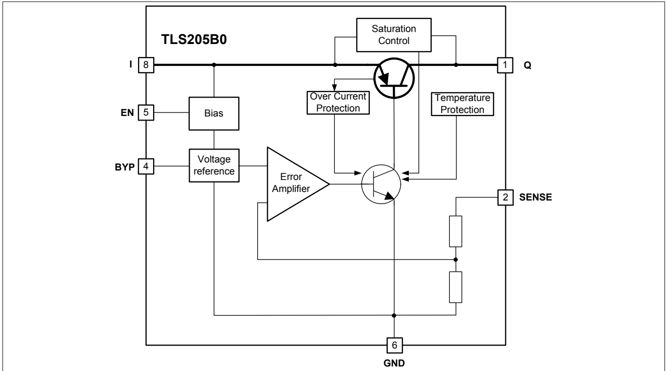
Figure 1 Block Diagram TLS205B0EJV50
