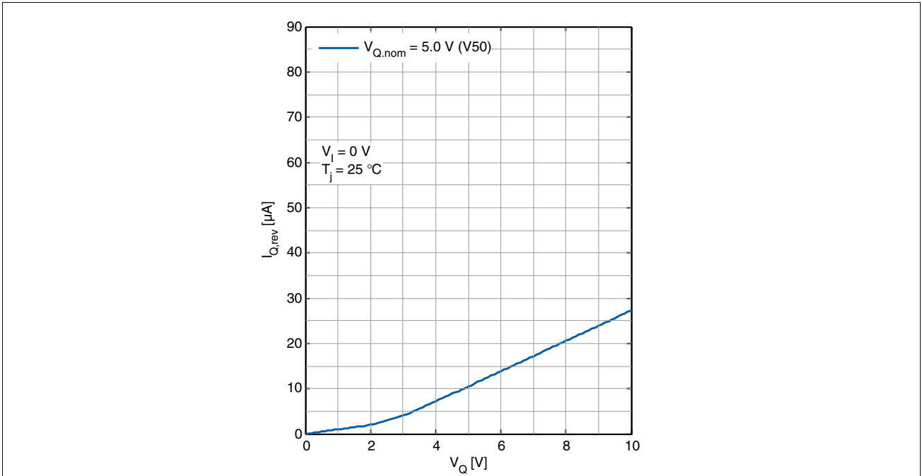
Figure 6 Reverse Output Current
