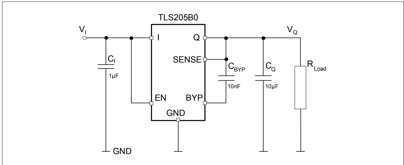
Figure 3 Typical Application Circuit TLS205B0EJV50
