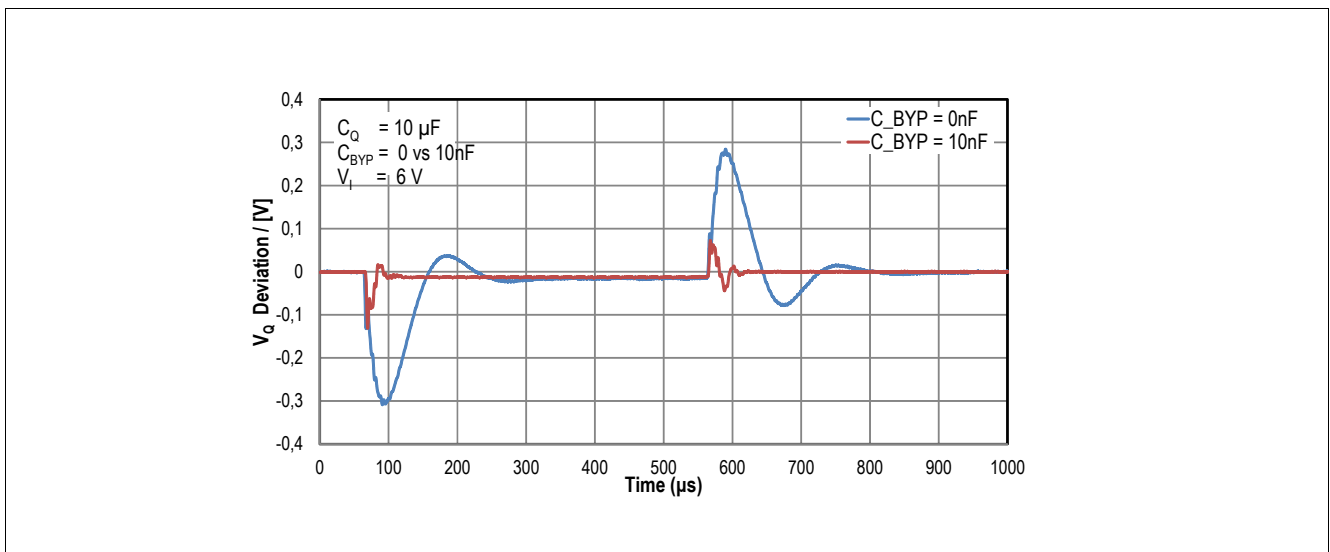
Figure 5 Influence of C_{BYP} : example of transient response to one and the same load step with and without C_{BYP} of 10 nF ( I_Q : 100 mA to 500 mA)
