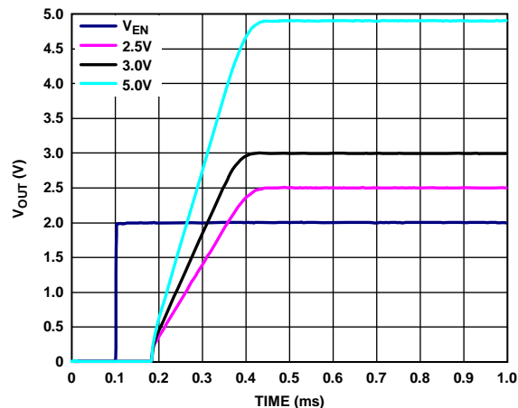
Figure 62. Typical Start-Up Behavior
