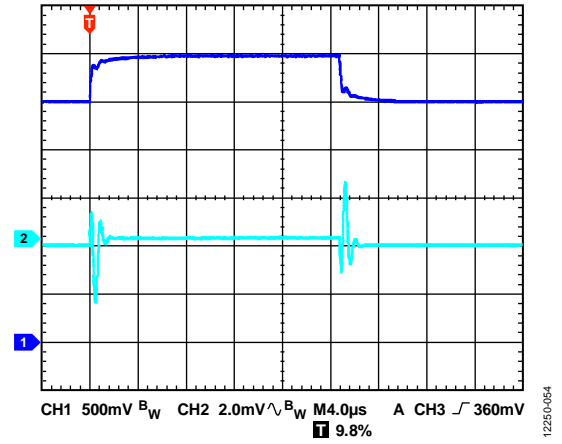
Figure 54. Line Transient Response, 2.5 V to 3 V, I_{LOAD} = 500 mA, Adjustable Version, V_{OUT} = 1.2 V, CH1 = V_{IN} , CH2 = V_{OUT}
