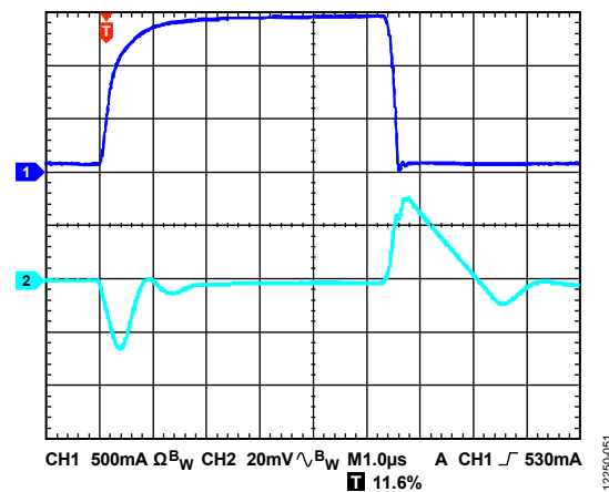
Figure 51. Load Transient Response, I_{LOAD} = 100mA to 1.6A , Adjustable Version, V_{OUT} = 1.2V , V_{IN} = 2.5V , CH1 = I_{LOAD} , CH2 = V_{OUT}
