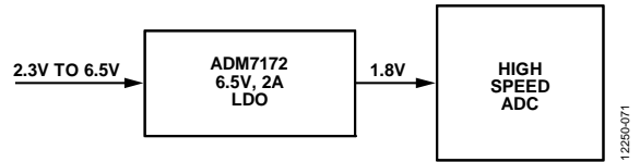
Figure 70. High Speed ADC Power
