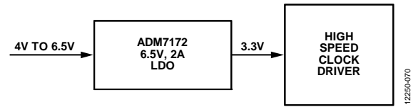
Figure 69. Clock Driver Power
