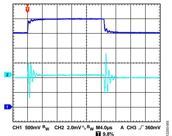
Figure 55. Line Transient Response, 2.5 V to 3 V, I_{LOAD} = 2 A, Adjustable Version, V_{OUT} = 1.2 V, CH1 = V_{IN} , CH2 = V_{OUT}
