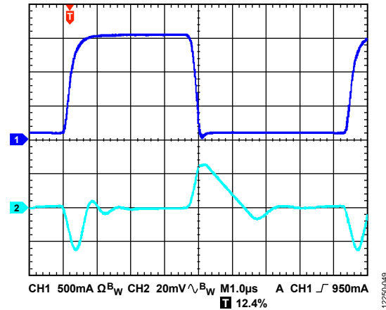
Figure 49. Load Transient Response, I_{LOAD} = 100mA to 1.6A , V_{OUT} = 5V , V_{IN} = 5.5V , CH1 = I_{LOAD} , CH2 = V_{OUT}
