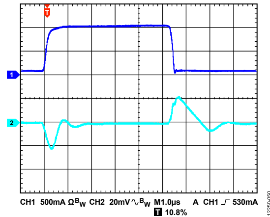
Figure 50. Load Transient Response, I_{LOAD} = 10mA to 1A , Adjustable Version, V_{OUT} = 1.2V , V_{IN} = 2.5V , CH1 = I_{LOAD} , CH2 = V_{OUT}
