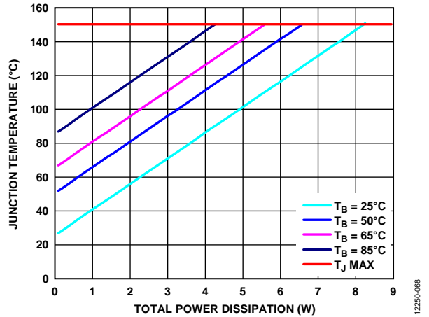
Figure 68. LFCSP Power Dissipation for Various Board Temperatures
