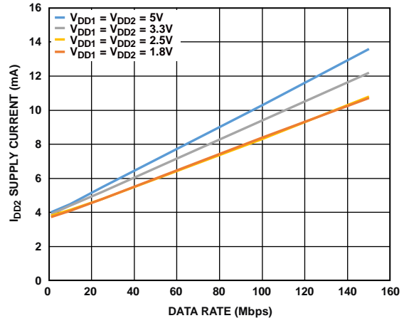
Figure 14. ADuM141D/ADuM141E I_{DD2} Supply Current vs. Data Rate at Various Voltages
