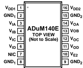
Figure 6. ADuM140E Pin Configuration
