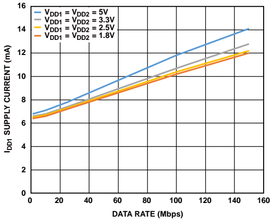
Figure 11. ADuM140D/ADuM140E I_{DD1} Supply Current vs. Data Rate at Various Voltages
