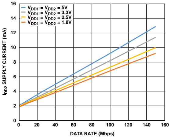
Figure 12. ADuM140D/ADuM140E I_{DD2} Supply Current vs. Data Rate at Various Voltages
