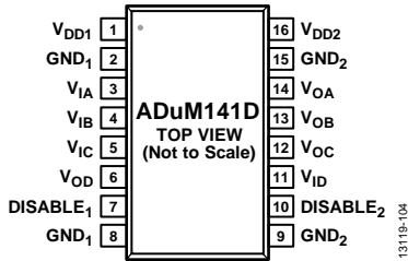
Figure 7. ADuM141D Pin Configuration
