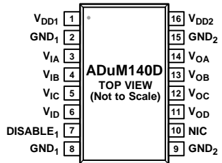
Figure 5. ADuM140D Pin Configuration
