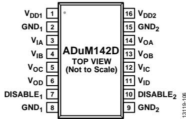
Figure 9. ADuM142D Pin Configuration
