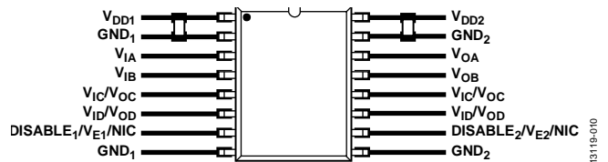
Figure 19. Recommended Printed Circuit Board Layout
