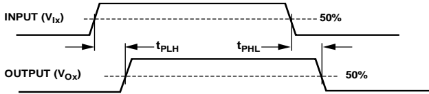
Figure 22. Propagation Delay Parameters
