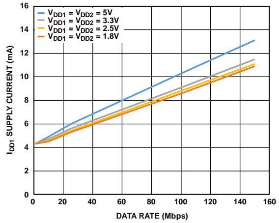
Figure 15. ADuM142D/ADuM142E I_{DD1} Supply Current vs. Data Rate at Various Voltages
