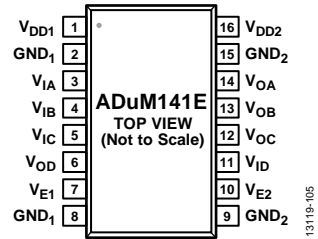
Figure 8. ADuM141E Pin Configuration
