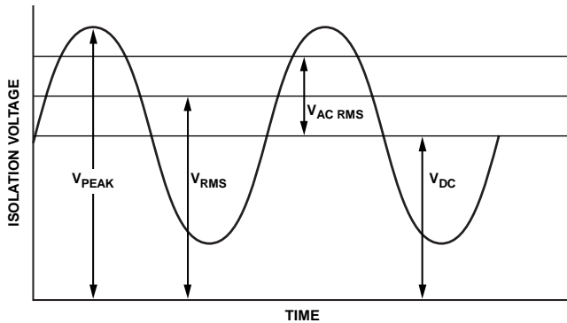
Figure 24. Critical Voltage Example
