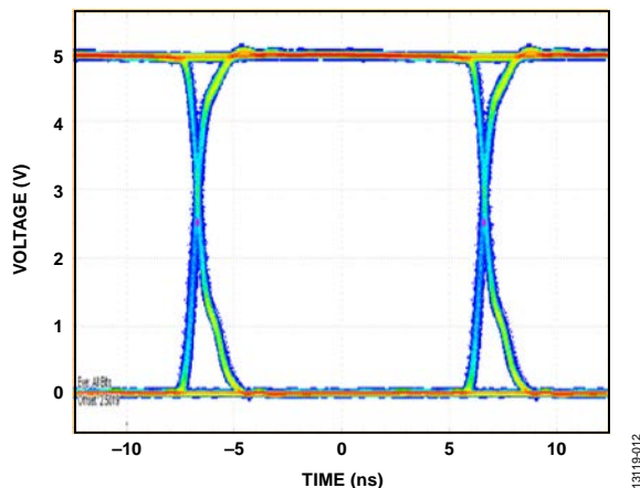
Figure 23. ADuM140D/ADuM140E/ADuM141D/ADuM141E/ADuM142D/ADuM142E Eye Diagram
