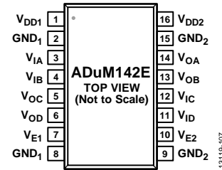
Figure 10. ADuM142E Pin Configuration
