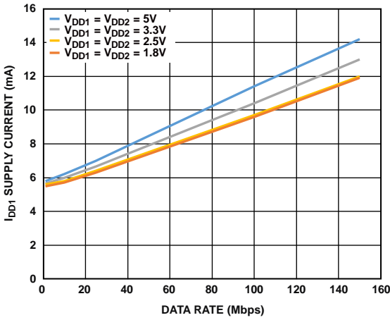
Figure 13. ADuM141D/ADuM141E I_{DD1} Supply Current vs. Data Rate at Various Voltages
