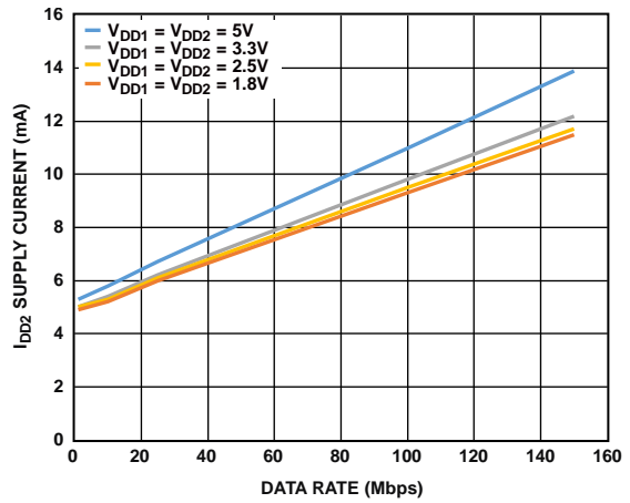
Figure 16. ADuM142D/ADuM142E I_{DD2} Supply Current vs. Data Rate at Various Voltages
