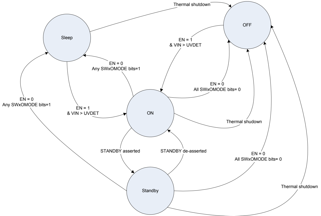
Figure 9. State Diagram
