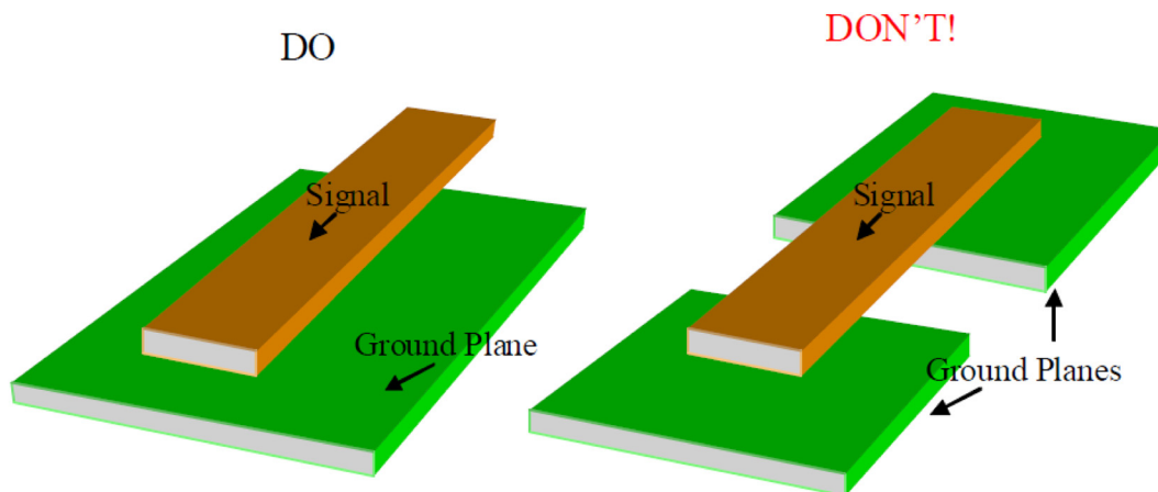
Figure 23. Recommended Shielding for Critical Signals
