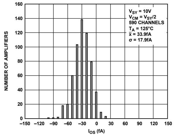
Figure 39. Input Offset Current Histogram
