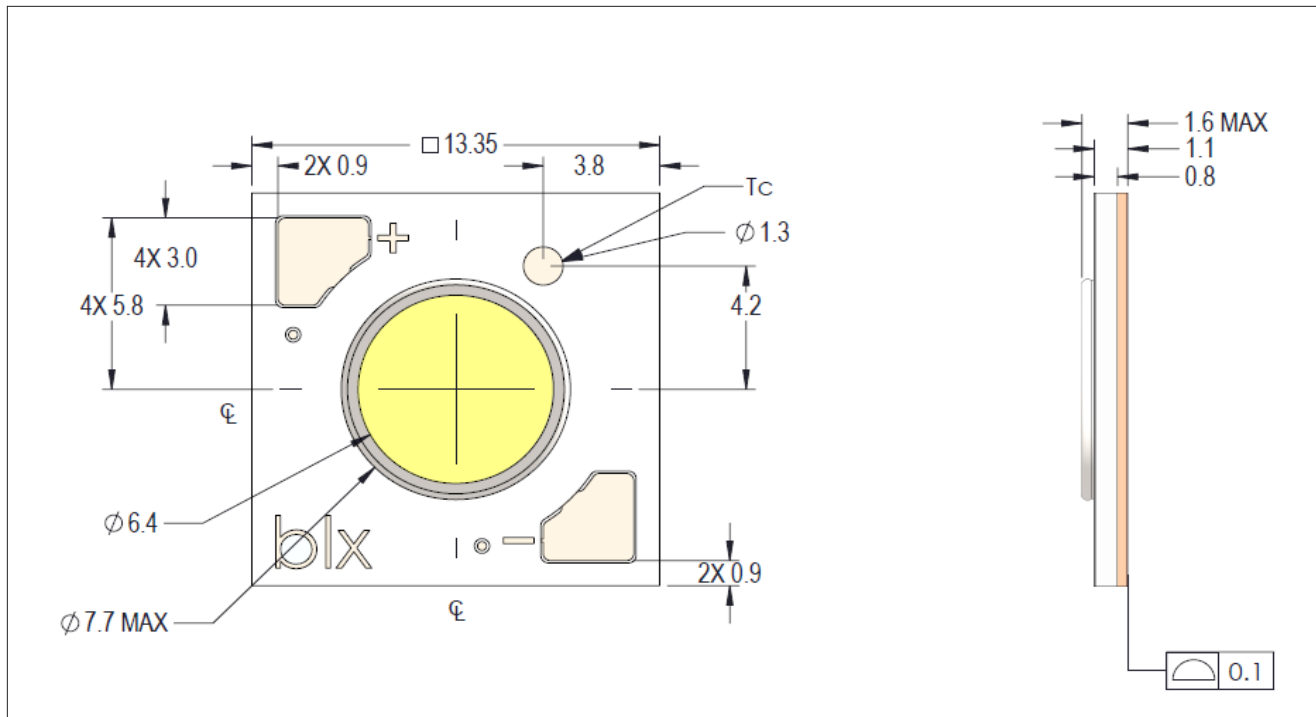
Figure 9: Drawing for H6 LED Array
