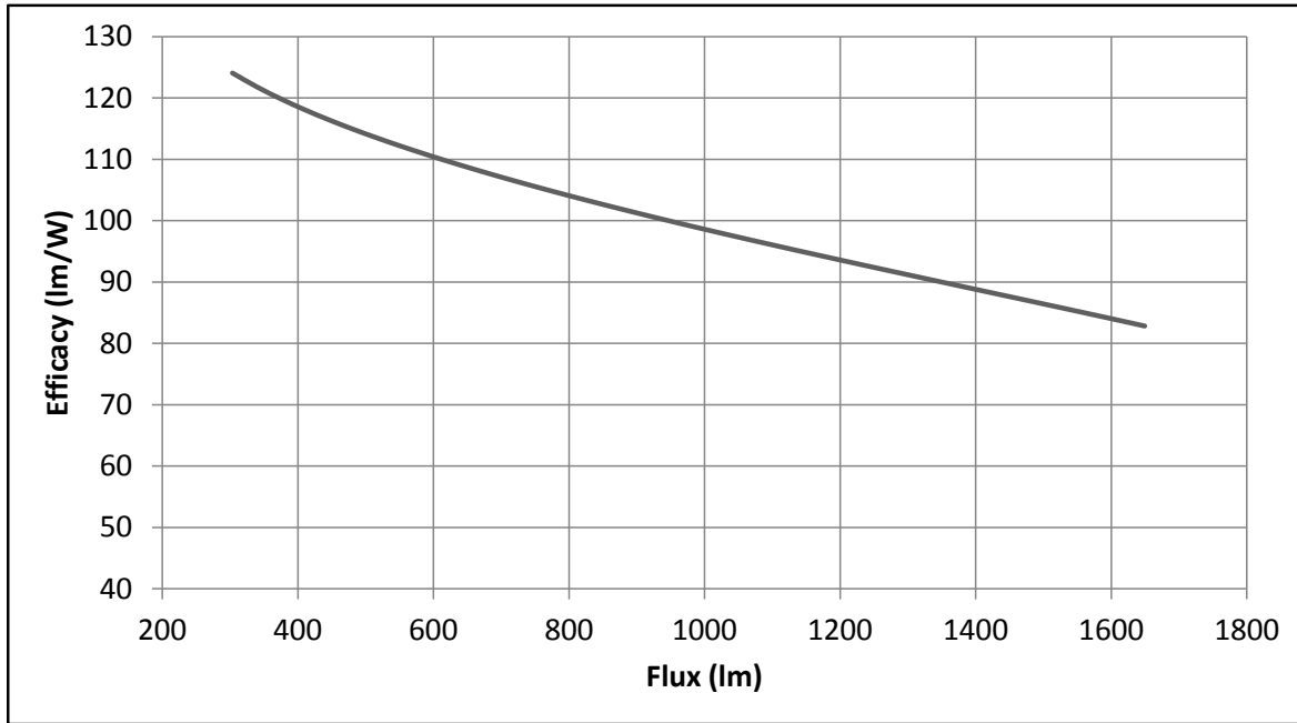
Figure 1: Efficacy vs. Flux ( T_j = T_c = 25^\circ\text{C} ; BXRH-30E1000-C-23)
