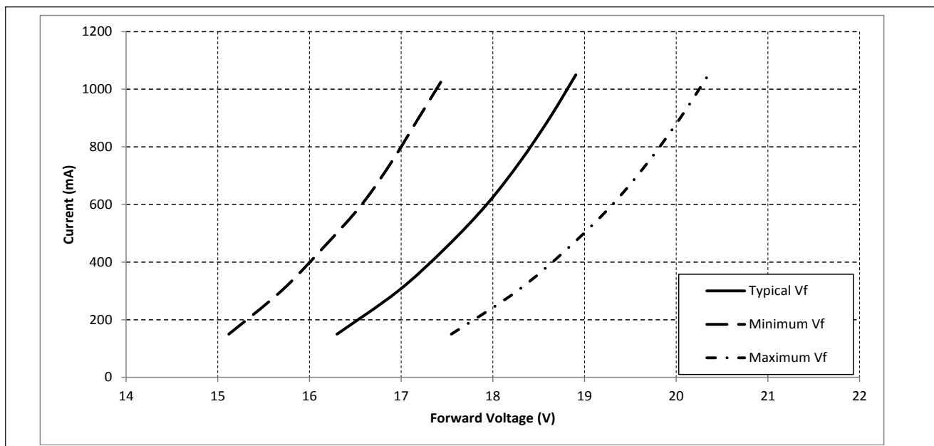
Figure 2: Drive Current vs. Voltage ( T_j = T_c = 25^\circ\text{C} )
