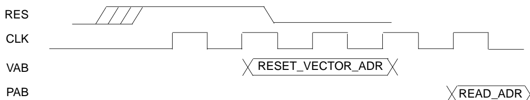
Figure 5-19 Reset Interface
