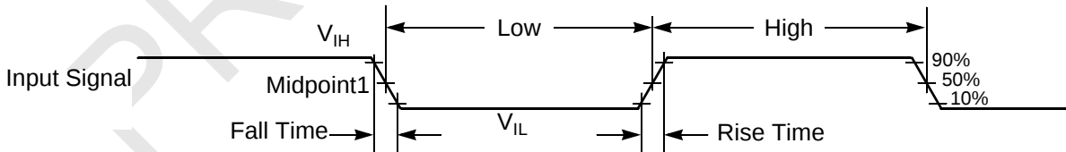
Figure 10-2 Input Signal Measurement References
