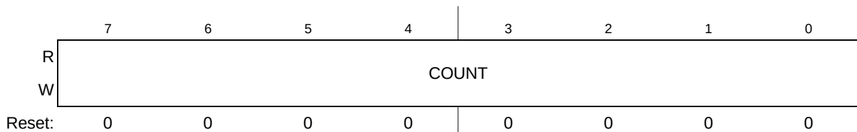
Figure 26-10. PWM Counter Registers (PWMCNT n )
