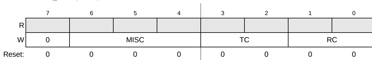
Figure 31-7. UART Command Registers (UCR n )
