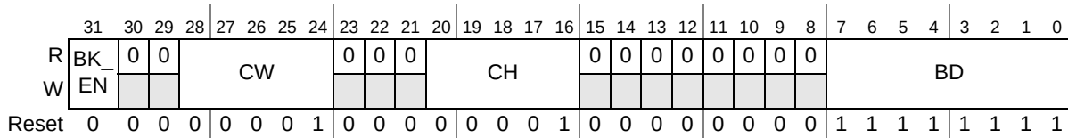
Figure 22-6. LCD Cursor Width Height and Blink Register (LCD_CWHB)
