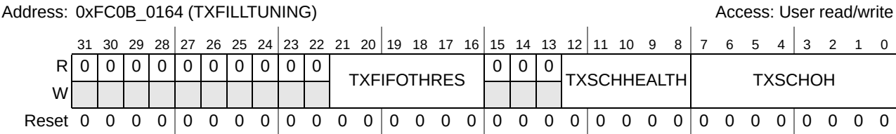
Figure 21-25. Transmit FIFO Tuning Controls (TXFILLTUNING)
