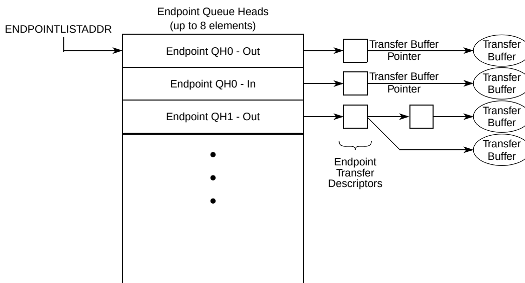
Figure 21-38. End Point Queue Head Organization
