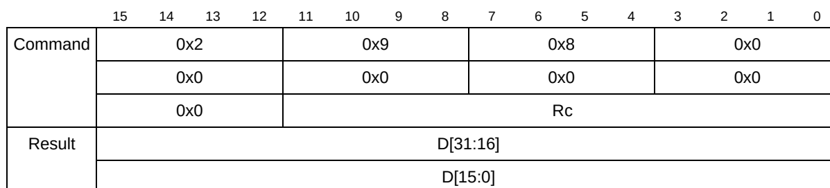
Figure 36-35. RCREG Command/Result Formats
