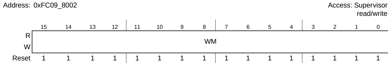
Figure 27-3. Watchdog Modulus Register (WMR)
