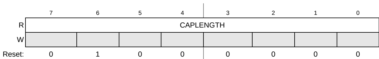
Figure 21-10. Capability Registers Length Register (CAPLENGTH)
