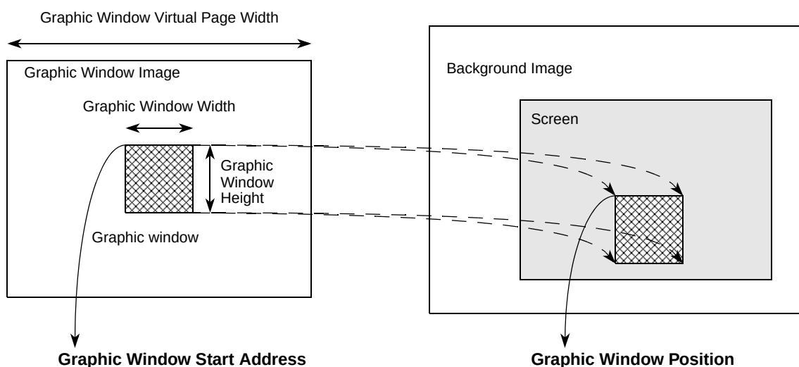
Figure 22-28. Graphic Window on Screen
