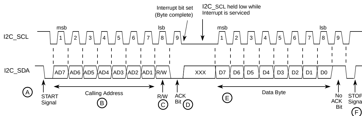
Figure 32-7. I 2 C Standard Communication Protocol
