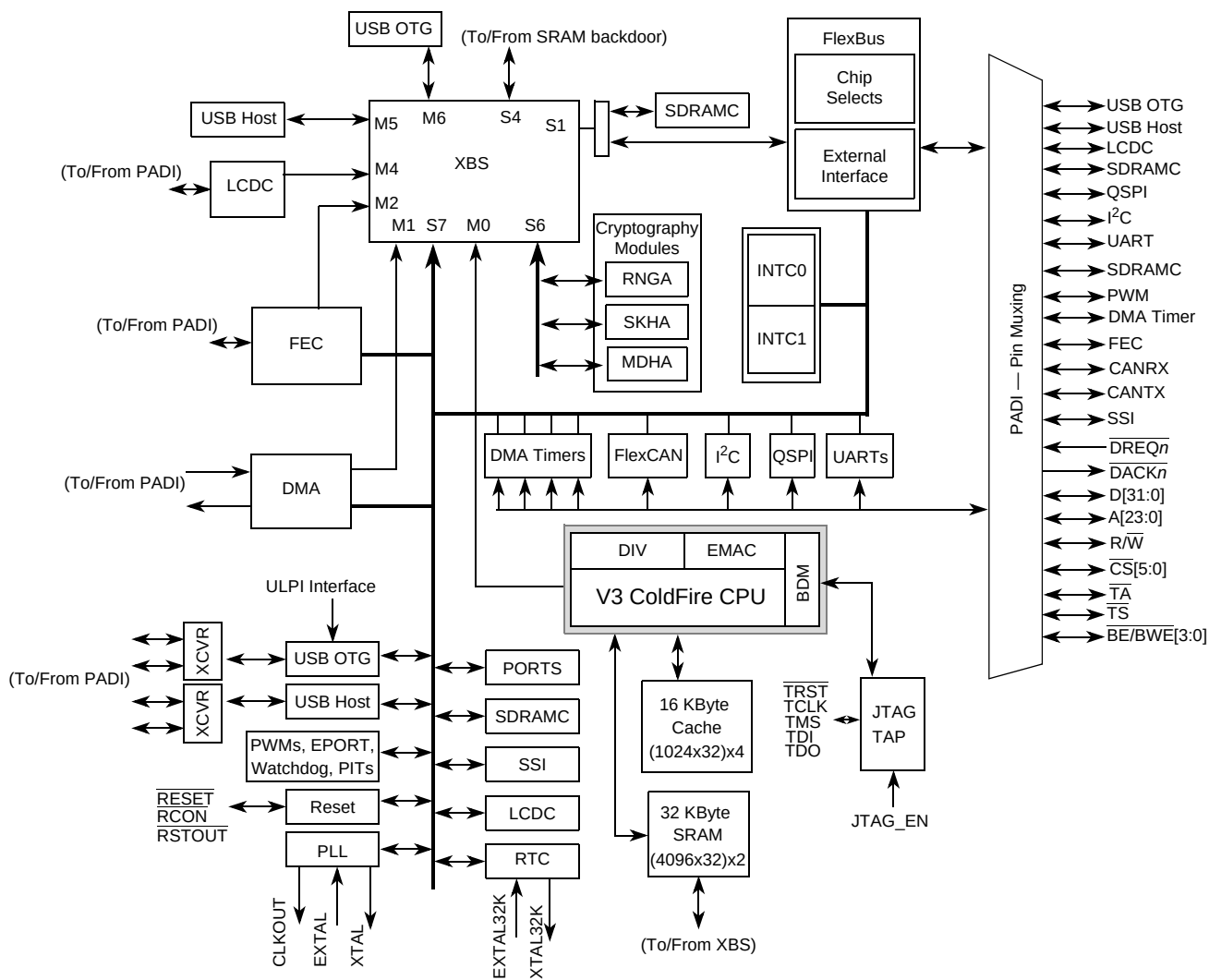
Figure 1-1. MCF5329 Block Diagram
