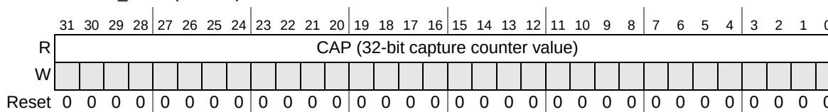
Figure 29-6. DTCRn Registers
