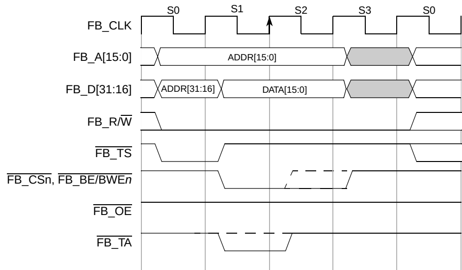
Figure 17-14. Single Word-Write Transfer
