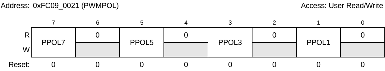
Figure 26-3. PWM Polarity Register (PWMPOL)
