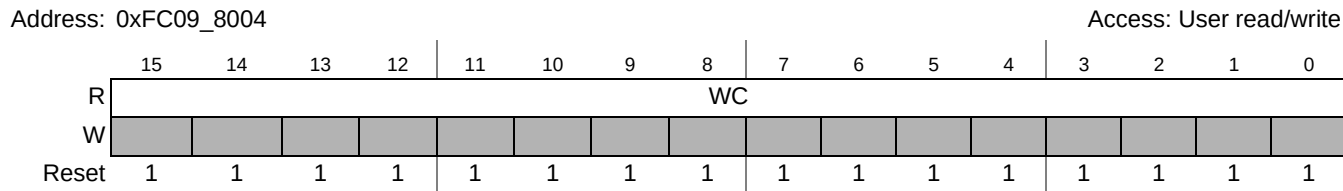
Figure 27-4. Watchdog Count Register (WCNTR)
