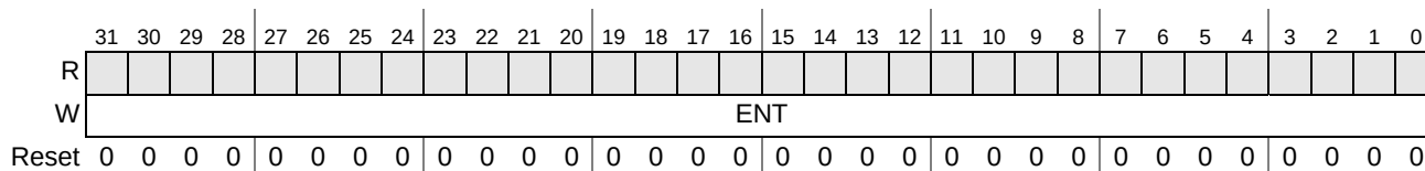
Figure 34-3. RNG Entropy Register (RNGER)
