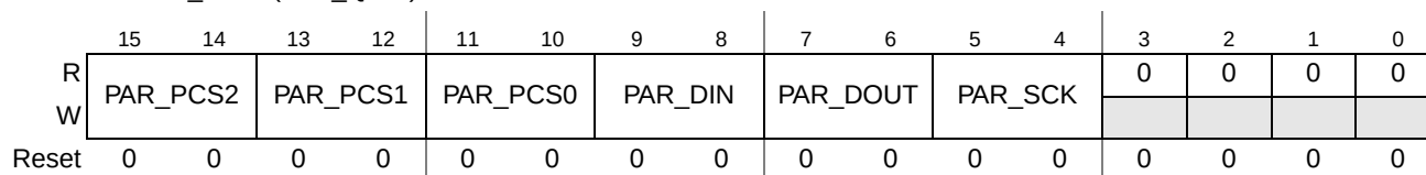
Figure 13-38. QSPI Pin Assignment (PAR_QSPI)
