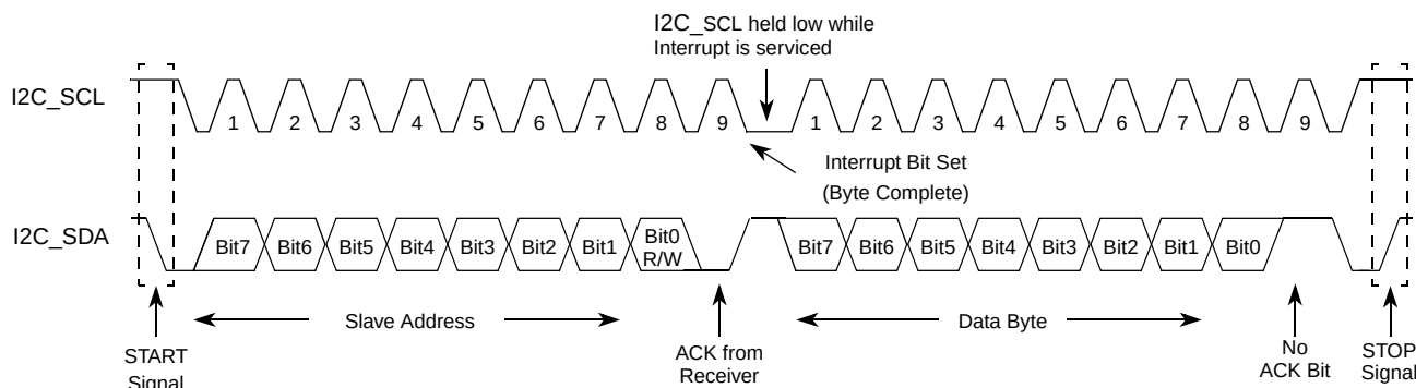
Figure 32-8. Data Transfer
