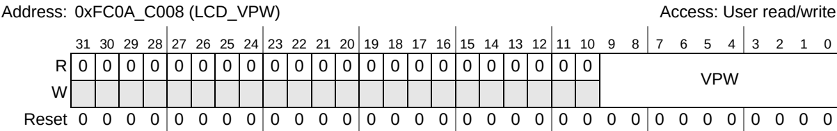
Figure 22-4. LCD Virtual Page Width Register (LCD_VPW)
