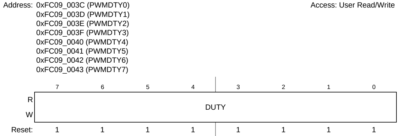
Figure 26-12. PWM Duty Registers (PWMDTY n )
