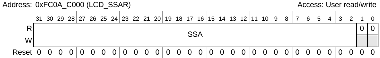
Figure 22-2. LCD Screen Start Address Register (LCD_SSAR)
