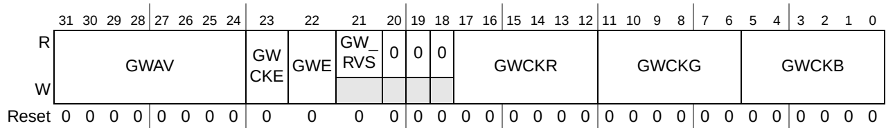
Figure 22-25. LCD Graphic Window Control Register (LCD_GWCR)
