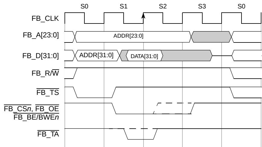
Figure 17-15. Longword-Read Transfer
