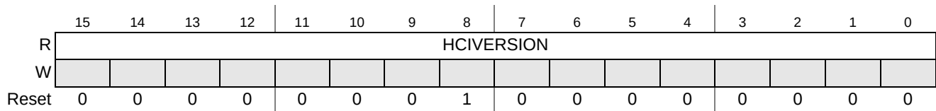
Figure 21-9. Host Controller Interface Version Register (HCVERSION)
