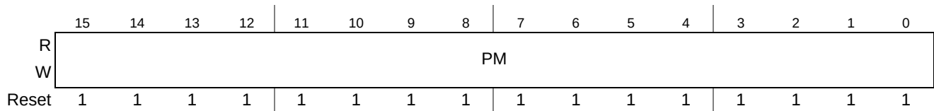
Figure 28-3. PIT Modulus Register (PMRn)
