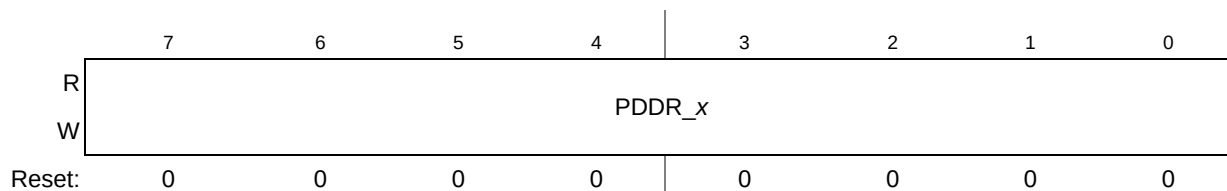
Figure 13-11. Port Data Direction Registers (PDDR_x)
