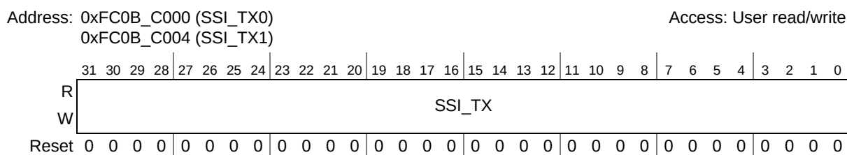
Figure 24-4. SSI Transmit Data Registers (SSI TX0, SSI TX1)
