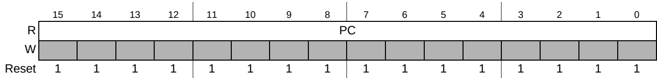
Figure 28-4. PIT Count Register (PCNTRn)
