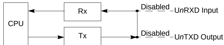
Figure 31-22. Local Loopback
