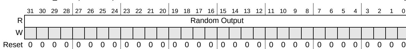
Figure 34-4. RNGOUT
