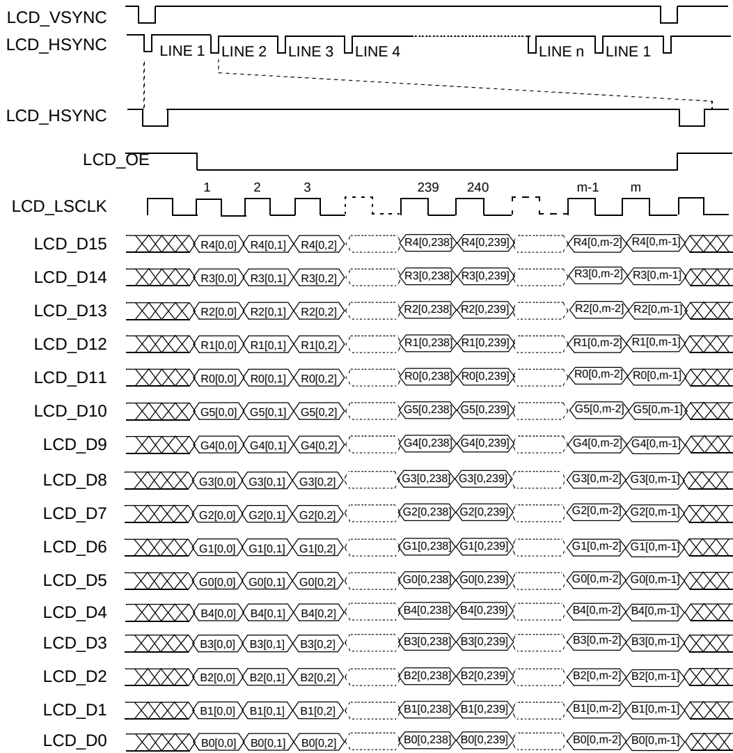
Figure 22-40. LDC Interface Timing for Active Matrix Color Panels
