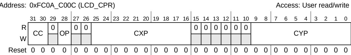
Figure 22-5. LCD Cursor Position Register (LCD_CPR)
