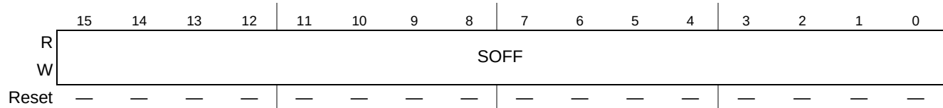
Figure 16-20. TCDn Signed Source Address Offset (TCDn_SOFF)
