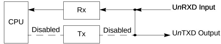
Figure 31-21. Automatic Echo
