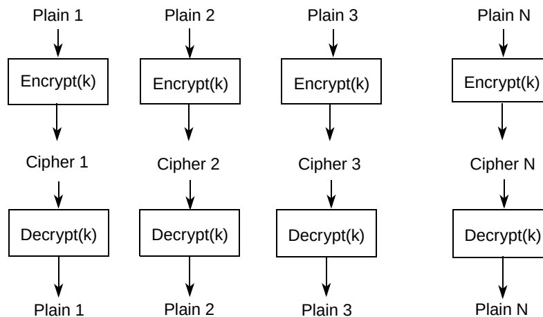
Figure 35-4. ECB Mode Processing
