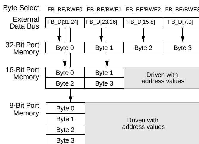
Figure 17-4. Connections for External Memory Port Sizes (CSCR n [SBM] = 0)
