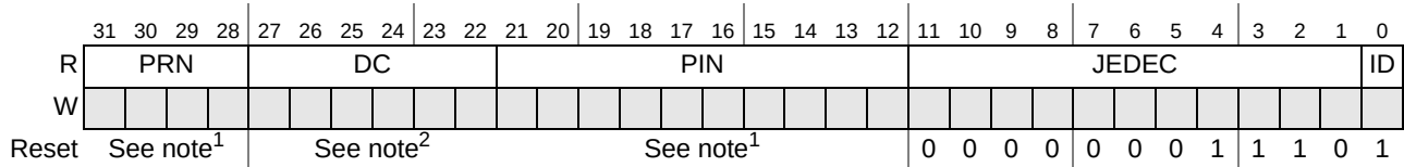
Figure 37-3. IDCODE Register
