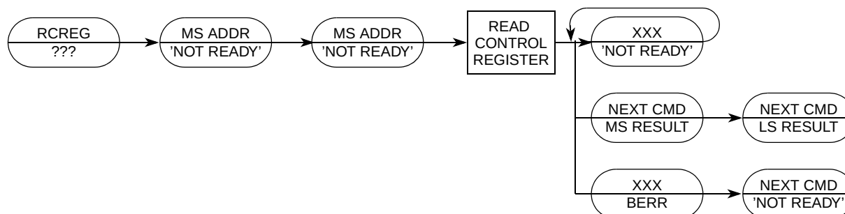
Figure 36-36. RCREG Command Sequence
