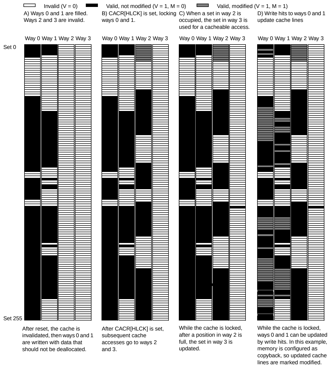
Figure 5-8. Cache Locking
