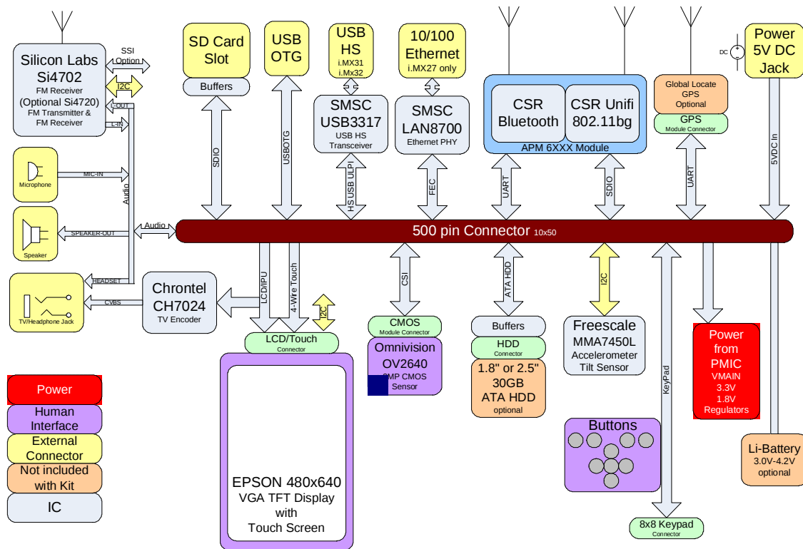
Figure 4-2 Functional Block 2 of 3
