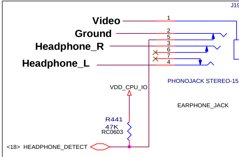
Figure 5-1 TV/Headphone Jack Pin-out and Schematics
