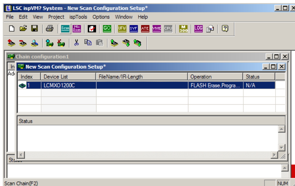
Figure 4-4 Scan CPLD Devices
