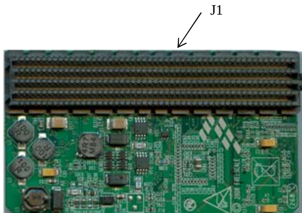
Figure 2-5 CPU Engine Board, Bottom View
